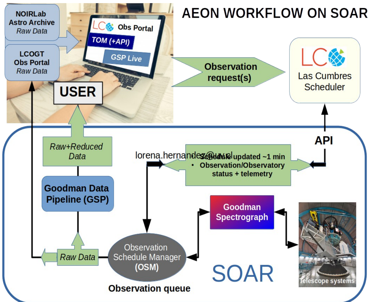
Figure 1: The AEON workflow on SOAR
