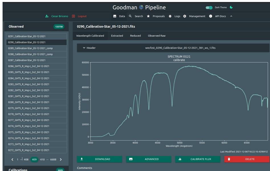
Figure 5: Reduced spectrum of a spectrophotometric standard star produced by the GSP
