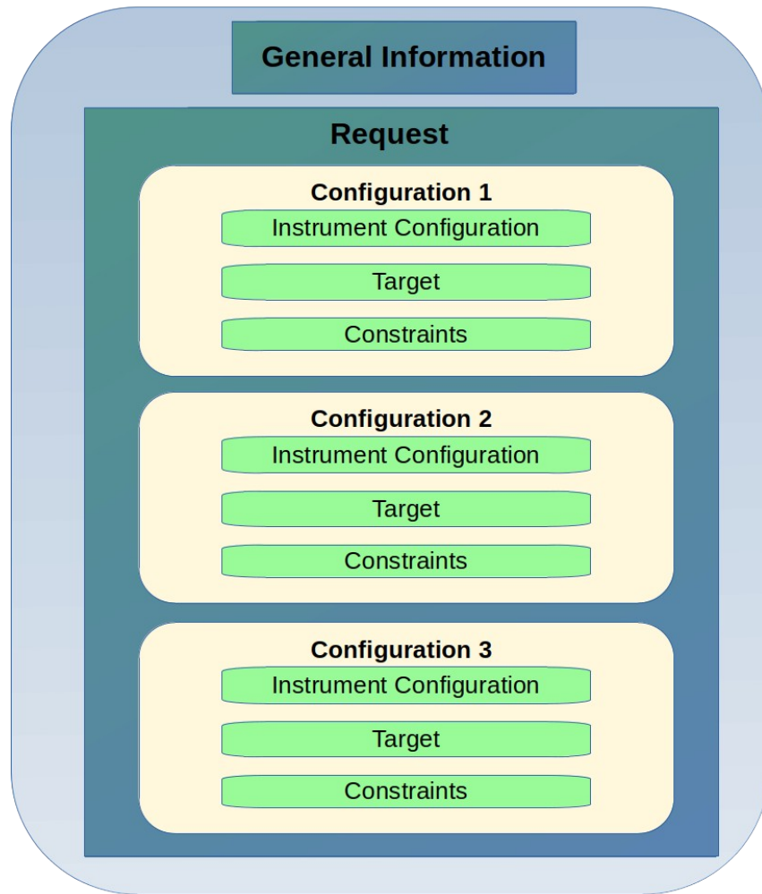
Figure 4: Schematic of the main elements of a Las Cumbres Observation Request
