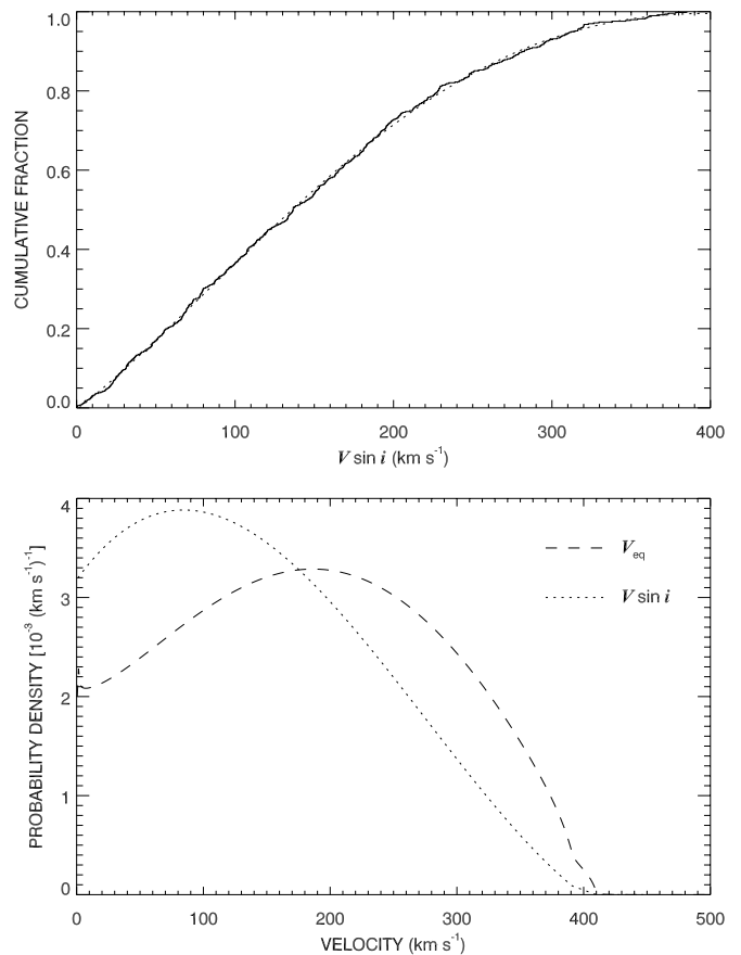
FIG. 6.—Top panel: Cumulative distribution function of V \sin i for the entire sample of 496 stars (solid line) and its polynomial fit (dotted line). Bottom panel: The V \sin i distribution derived from the polynomial fit (dotted line) and the associated distribution of equatorial velocity V_{\text{eq}} (dashed line).
