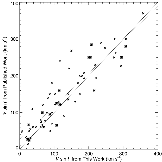
Fig. 2.—Comparison of our measured V \sin i values with published work. The solid line shows the one-to-one relationship, while the dotted line is the result of a linear least-squares fit.
