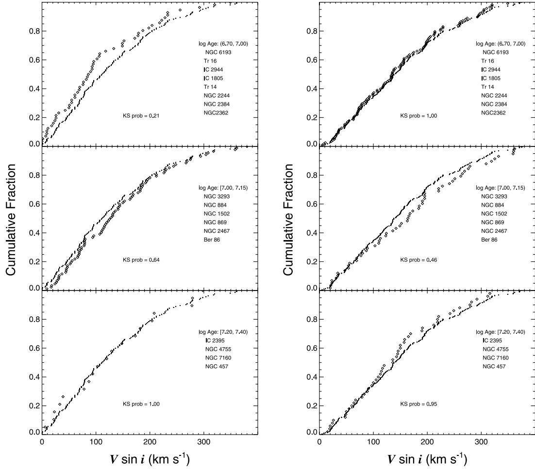
FIG. 8.—Cumulative distribution functions of V \sin i for the subgroups of high-mass ( M \geq 9 M_{\odot} , left panels) and low-mass ( M < 9 M_{\odot} , right panels) stars at different ages (increasing from top to bottom). Each panel has two curves: one is the function for the specific-age subgroup (diamonds) while the other is the function for all the stars of the three panels together (filled circles). The KS probability that the two samples are drawn from the same parent distribution is listed in each case.
