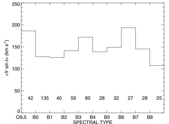
FIG. 3.—Mean V \sin i as a function of pseudospectral subtype. The number of stars in each subtype bin is given at the bottom.
