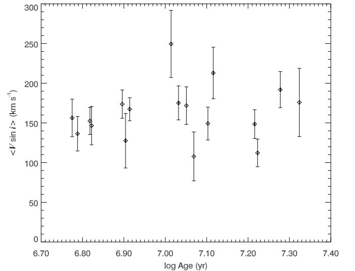
FIG. 10.—Mean V \sin i for stars ( M < 9 M_{\odot} ) in young clusters plotted against logarithm of cluster age.
