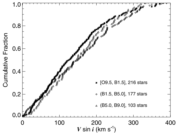
FIG. 4.—Cumulative distribution functions of V \sin i for the stars gathered into three groupings of pseudospectral subtype. The subtype range is given using the mathematical notation in which square brackets mean the boundary is included, while parentheses mean the boundary is not included.
