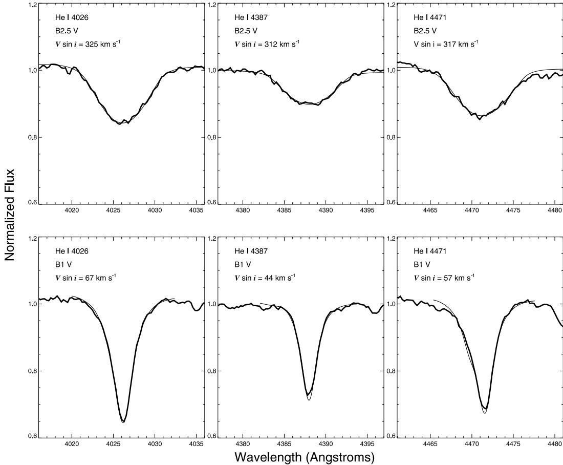
FIG. 1.— Fitting results for the He I lines ( thin lines ) compared with observed profiles ( thick lines ). The top panels show fits for a fast rotator, NGC 884 No. 2255, while the bottom panel shows the same for a slow rotator, NGC 884 No. 1983.
