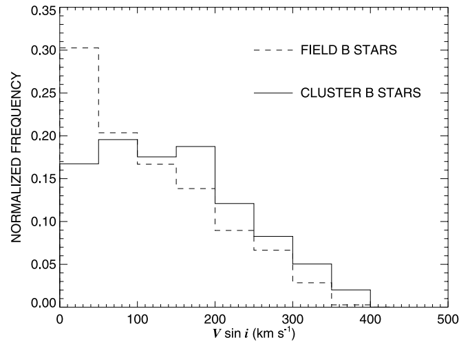
FIG. 5.—Histograms of V \sin i for field stars (Abt et al. 2002; dashed line) and for cluster stars (solid line).
