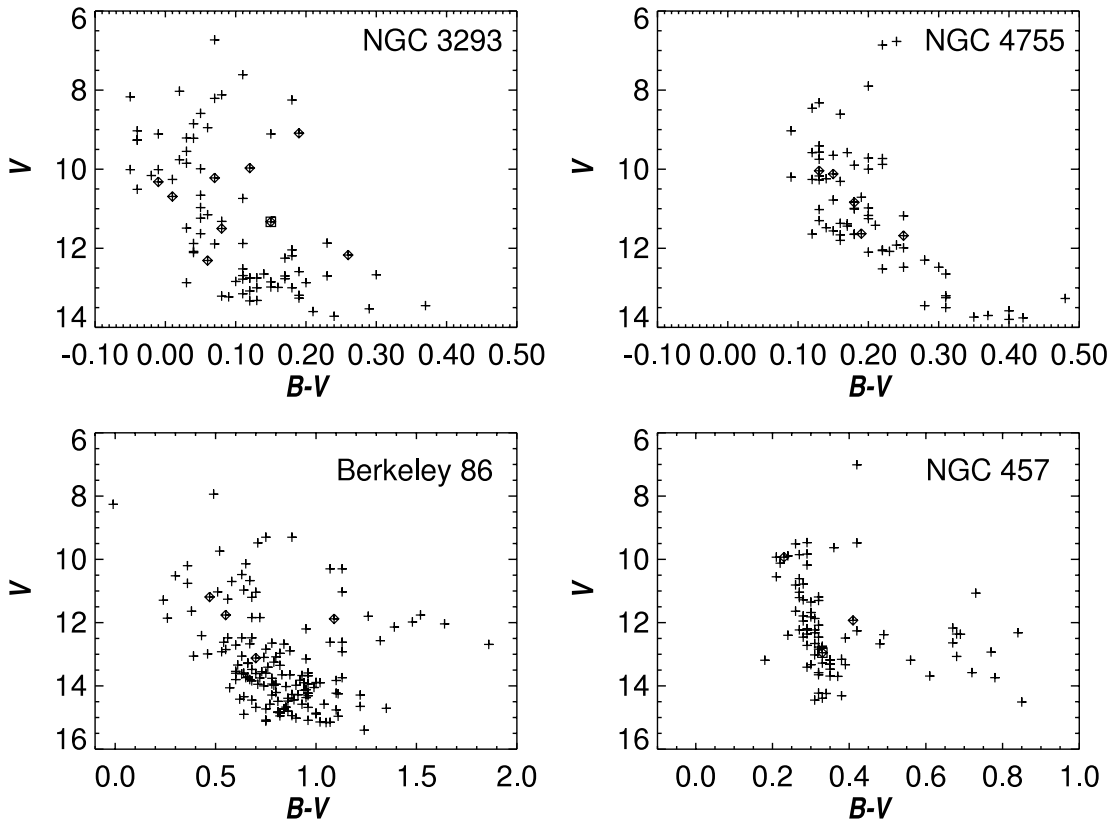
FIG. 11.—Color-magnitude diagrams for NGC 3293 (from photometry by Turner et al. 1980), Berkeley 86 (photometry by Forbes et al. [1992] and Massey et al. [1995]), NGC 4755 (photometry by Perry et al. [1976] and Dachs & Kaiser [1984]), and NGC 457 (photometry by Pesch [1959] and Hoag et al. [1961]). The crosses enclosed in diamonds mark the fast rotators ( V \sin i > 260 \text{ km s}^{-1} ). The only two candidate binary stars identified among the fast rotators are NGC 3293 No. 83 and NGC 457 No. 43, which are marked by enclosing squares.
