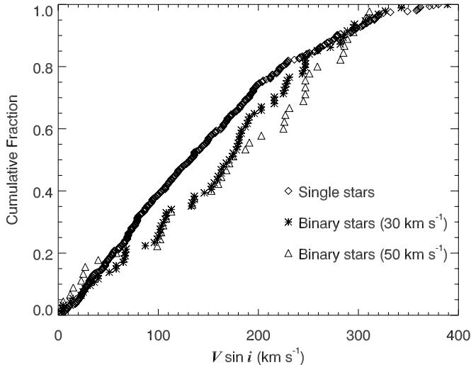
FIG. 7.— Cumulative distribution functions of V \sin i for single and candidate binary stars (according to two criteria for the minimum radial velocity range).
