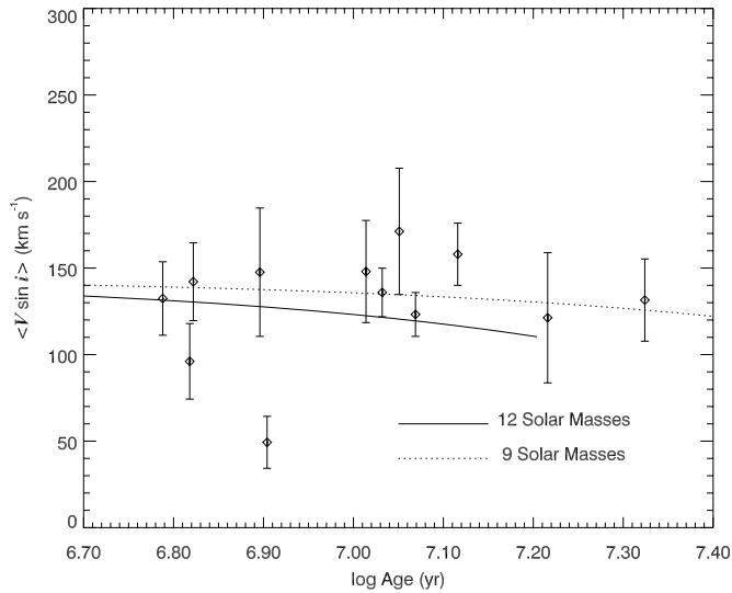
FIG. 9.—Mean V \sin i for high-mass stars ( M \geq 9 M_{\odot} ) in young clusters plotted against logarithm of cluster age. The solid and dotted lines show the prediction from Meynet & Maeder (2000) for an ensemble of 12 M_{\odot} and 9 M_{\odot} stars, respectively.
