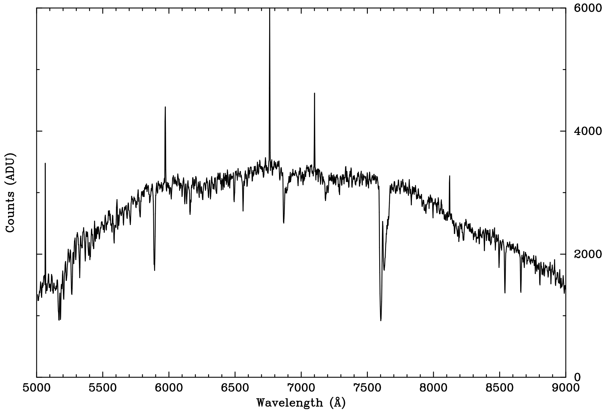
Extracted Spectrum UCAC3 73-7870 400M2
