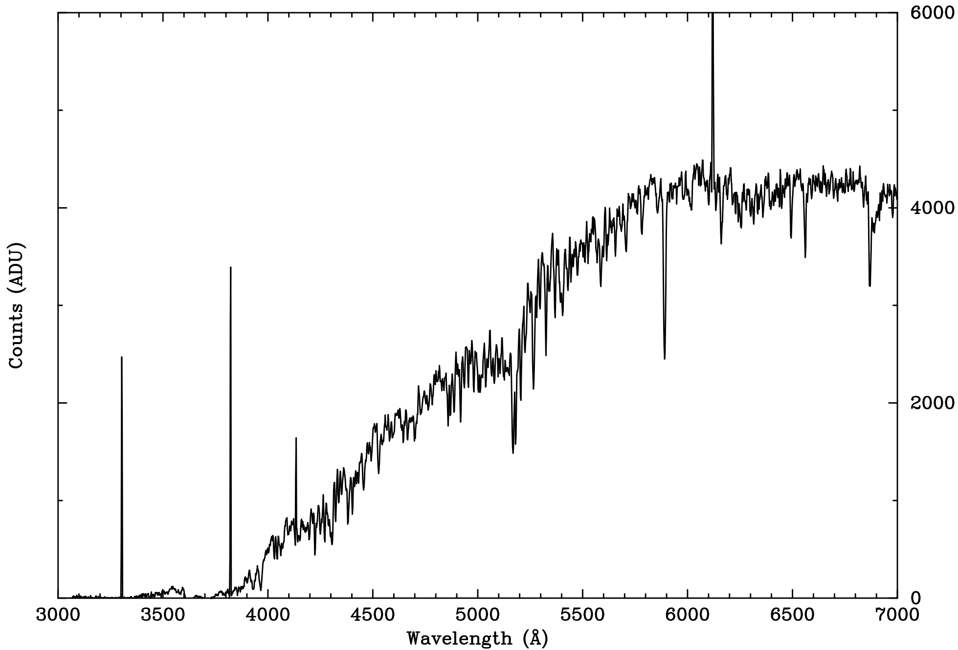
Extracted Spectrum UCAC3 73-7870 400M1
