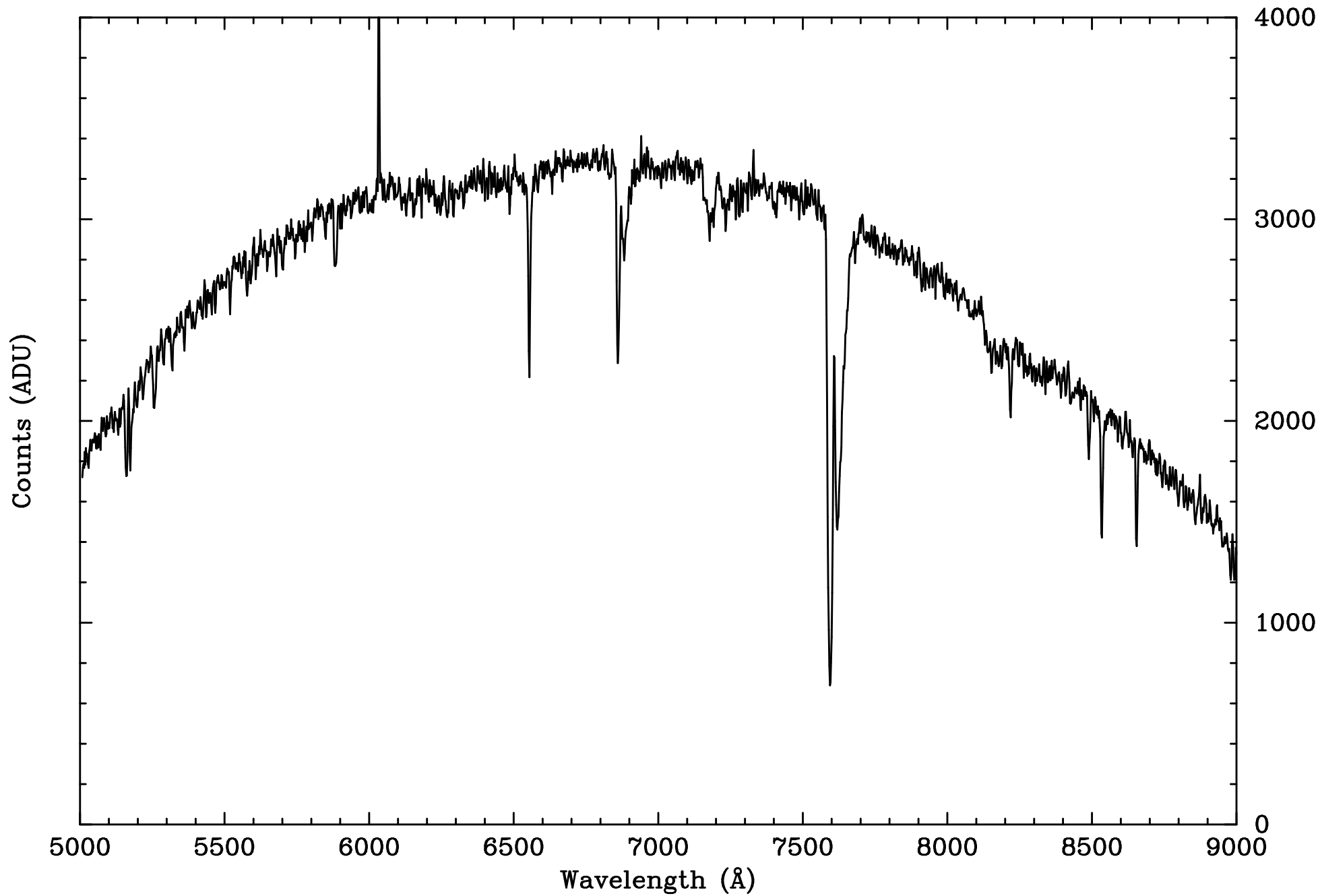
Extracted Spectrum IDK N002 400M2
