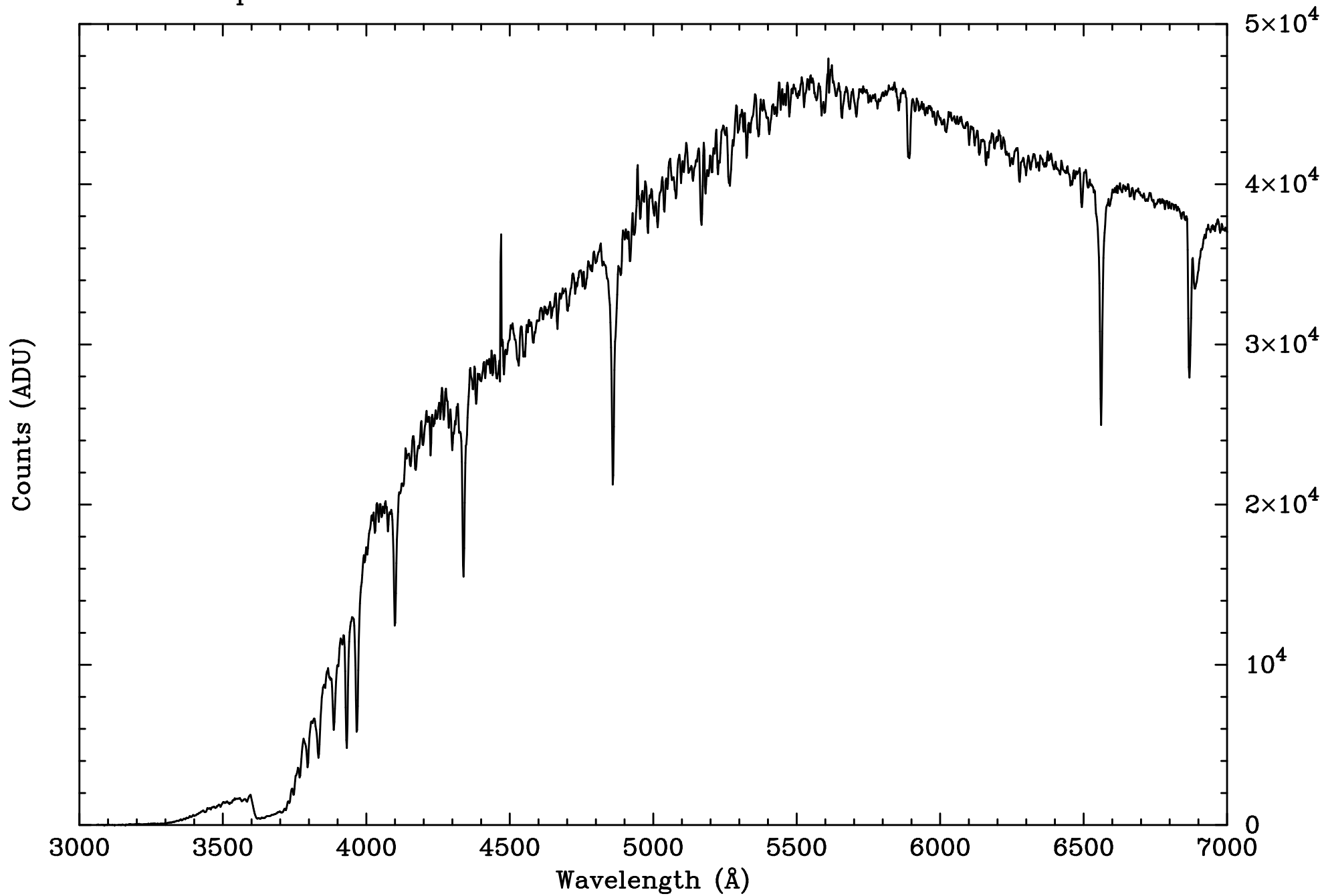
Extracted Spectrum 2MASS J0359-6732 400M1
