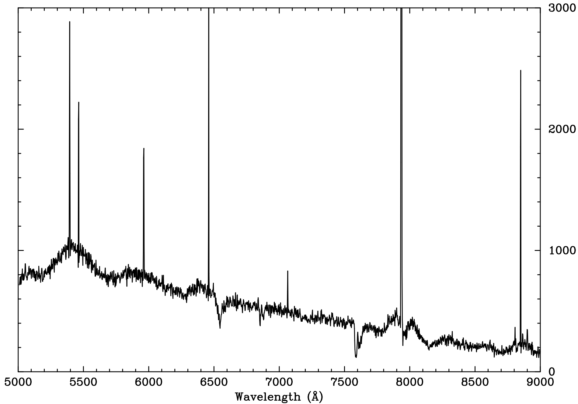
Extracted Spectrum PHL 1225 400M2
