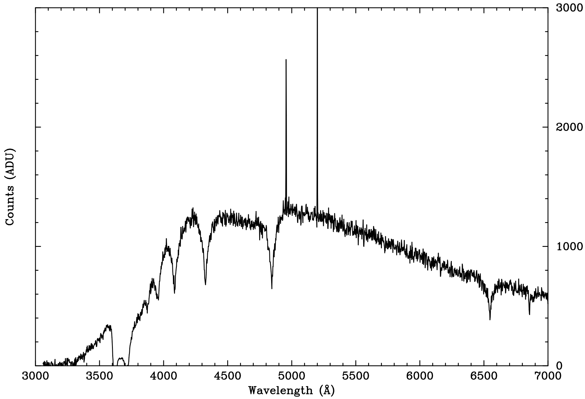
Extracted Spectrum PHL 1225 400M1
