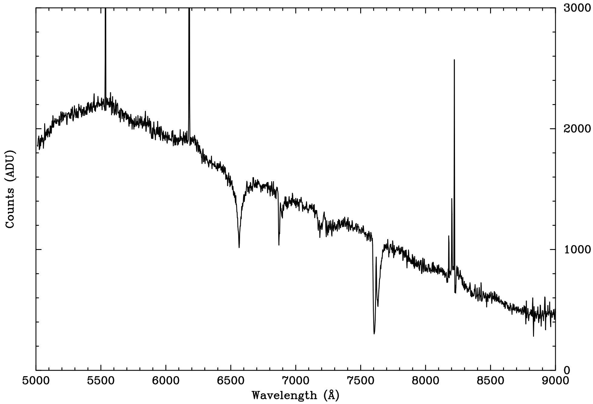
Extracted Spectrum PHL 1225 400M2
