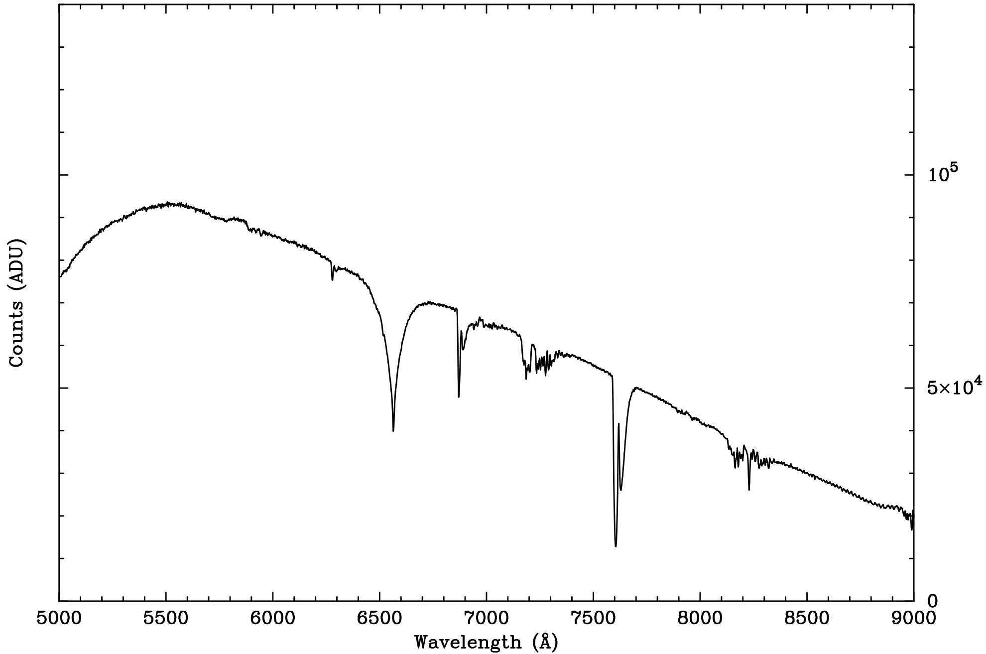
Extracted Spectrum EG 21 400M2
