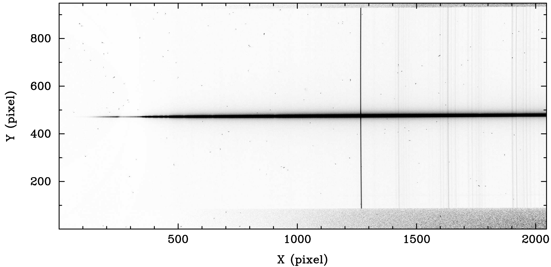
2MASS J0359-6732 400M1 1as Slit
