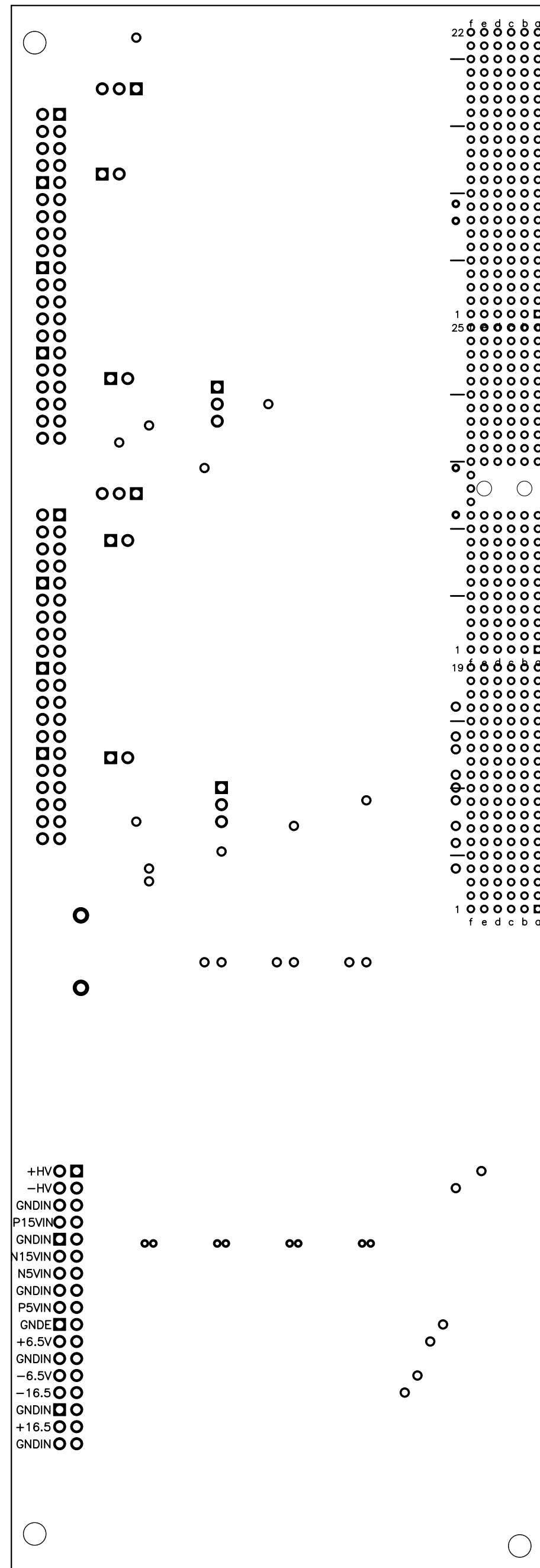
ASSEMBLY BOTTOM
