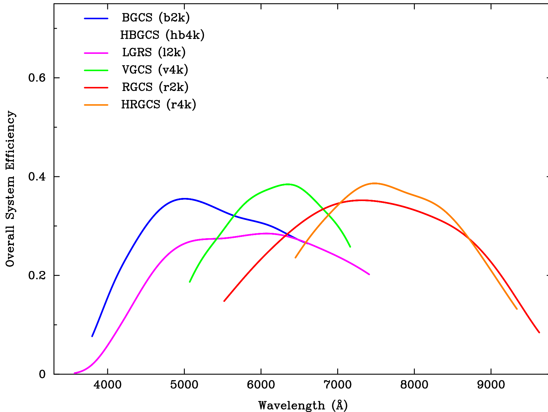
COSMOS System Throughput
