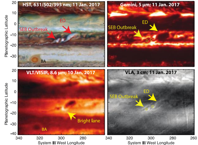
Figure 5: Jupiter South Equatorial Belt (SEB) outbreak of 2017, imaged at high resolution by HST, Gemini, VLT and the VLA. The various wavelengths are sensitive to different gasses and/or aerosols, and hence probe different depths and temperatures. From de Pater et al. 2019b, submitted.
