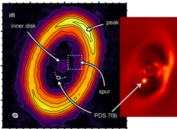
Figure 2: (Left) 870 \mu\text{m} ALMA continuum image of the PDS 70 disk with 0.07'' (8 AU) resolution (Keppler et al. 2018). (Right) VLT/SPHERE 1.6 \mu\text{m} image of the planet PDS 70b, located at the center of a dust-depleted gap as predicted by planet-disk interaction models (Müller et al. 2019). Fig. from Isella et al. 2019.
