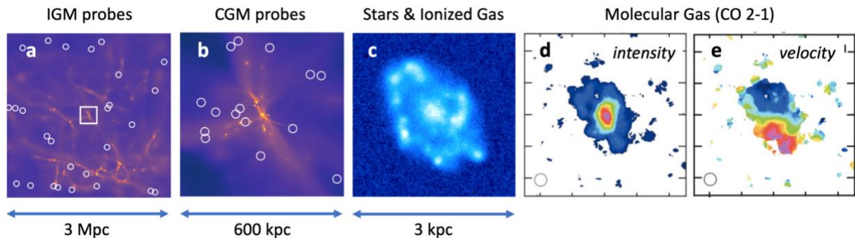
Figure 3: Together, observations with ELTs and the ngVLA will study critical components of the cosmic baryon cycle of galaxies at z \approx 2 (“cosmic noon”) from megaparsec environments to 100 pc scales characteristic of massive star-forming clusters. From left to right: (a, b) Multi-object spectrographs on GMT and TMT will measure intergalactic and circumgalactic gas (IGM, CGM) using UV absorption lines measured in the spectra of faint background galaxies. (c) AO imaging and integral field spectroscopy will observe stars and ionized gas with resolutions of order 150 pc. (d, e) The ngVLA will observe low- J transitions of CO at high angular resolution, tracing the detailed spatial and velocity structure of the fuel for star formation.
