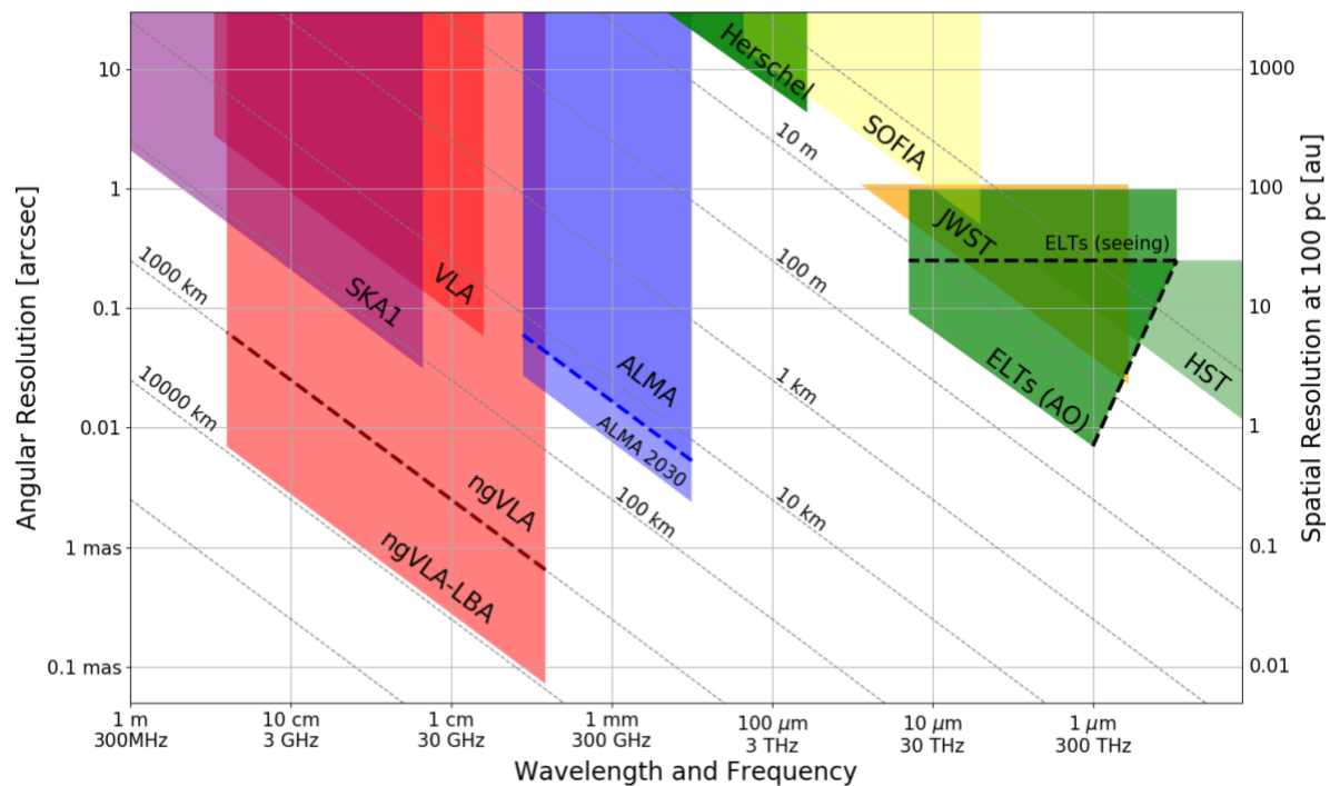
Figure 1: Angular resolution versus wavelength for current and future-generation facilities, including the Next Generation Very Large Array (ngVLA), 30m-class Extremely Large Telescopes (ELTs), and a possible future expansion of ALMA with maximum baselines up to 30 km (ALMA 2030). A dashed line separates the ngVLA main array from the continental-scale Long Baseline Array (LBA). For ELTs, the lower left envelope indicates diffraction-limited AO performance in the infrared, and dashed lines schematically indicate a transition to seeing-limited performance in the optical. The scale at right shows spatial resolution (in AU) for observations of forming planetary systems at a distance of 100 pc.
