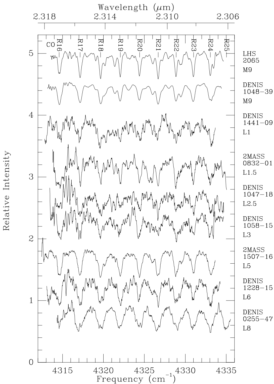
Figure 5. Spectra of a selection of very late M and L dwarfs spanning the L dwarf temperature range to L8.
