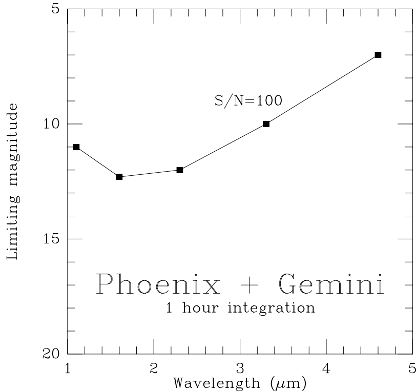
Figure 2. Approximate limiting magnitudes for signal-to-noise ratio 100 in a 1 hour integration for Phoenix on Gemini South. The values are based on sample spectra taken under good observing conditions at resolution 50000. This figure omits degradations to the signal-to-noise ratio due to blaze efficiency, seeing, cosmic rays, bad pixels, etc. In the thermal infrared the maximum exposure time for a single integration will be much less than 1 hour due to the contribution from the thermal background radiation. For instance, at 4.6 \mu\text{m} the maximum integration time for an individual exposure is about 2 minutes.
