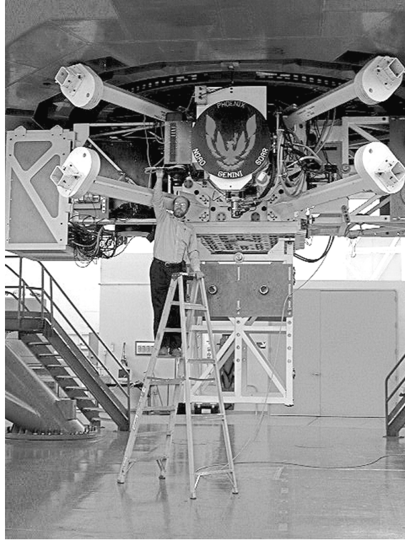
Figure 1. Phoenix mounted on the instrument support structure of Gemini South. K.H.H. is standing on the ladder under the instrument. Below his shoulder level is a standard Gemini instrument mounting frame for another instrument in the uplooking port. To his left, occupying a side looking port, is GCAL, the Gemini calibration unit. The end of the Phoenix dewar is prominent (behind the logo) with one cold head visible below the dewar. The four ‘legs’ are the balance weights required to match the weight and moment to the Gemini instrument specifications.
