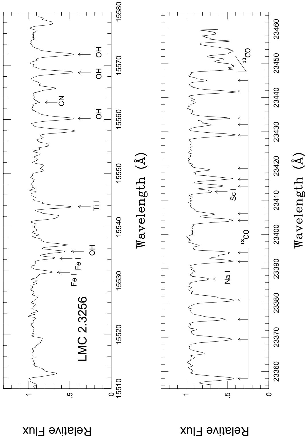
Figure 3. Sample spectra for the LMC red giant 2.3256 ( K=12.0 ; see Smith et al. 3 ) showing two different wavelength regions. Some stronger lines are identified. Each spectrum consists of a combination of three 30 minute integrations and the signal-to-noise in each spectrum is a bit more than 100.
