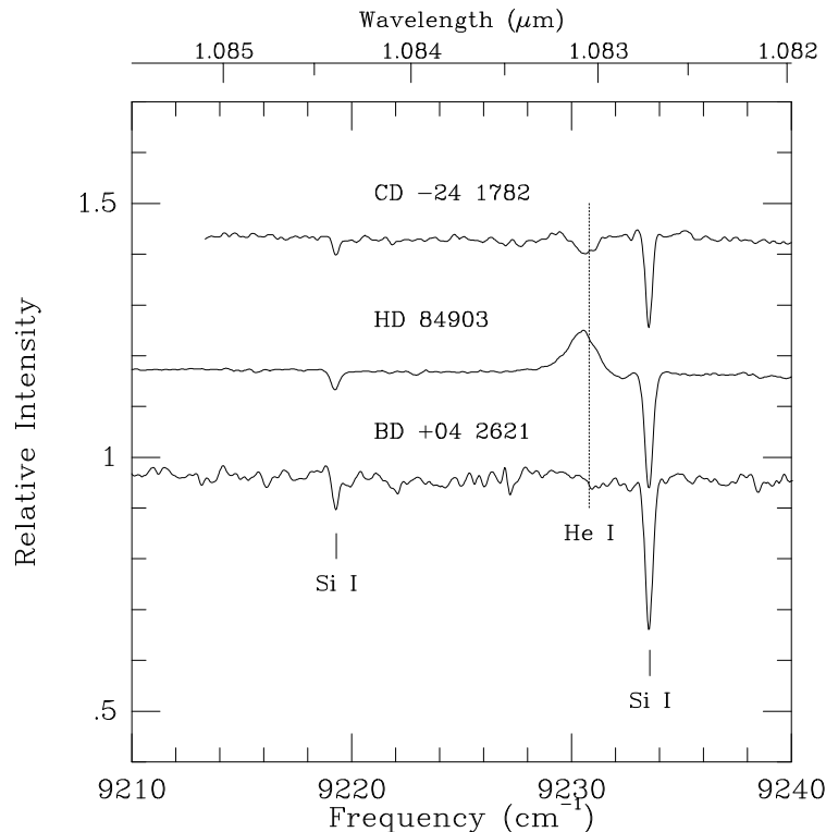
Figure 4. Spectra of three metal poor giant stars ( [Fe/H] \sim -2.5 ) at the He I 10830 Å line.
