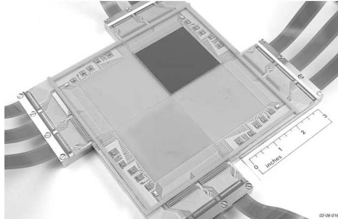
Fig. 5. A demonstration focal plane with four ORION modules. One module contains an InSb SCA while the others have bare readouts. This focal plane demonstrates the ability of the 2-sided buttable modules to create a 4K \times 4K focal plane.
