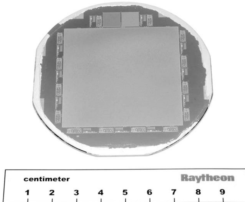
Fig. 2. Photograph of 82 mm diameter InSb wafer with a 2048 × 2048 (2K × 2K) element array patterned on it. Each detector element is 25 μm square. The small die surrounding the 2K × 2K array are various test structures.
