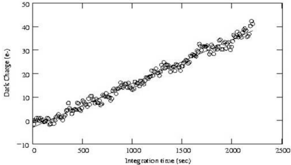
Fig. 10. Graph depicts "sample-up-the-ramp" technique for dark current measurements.
