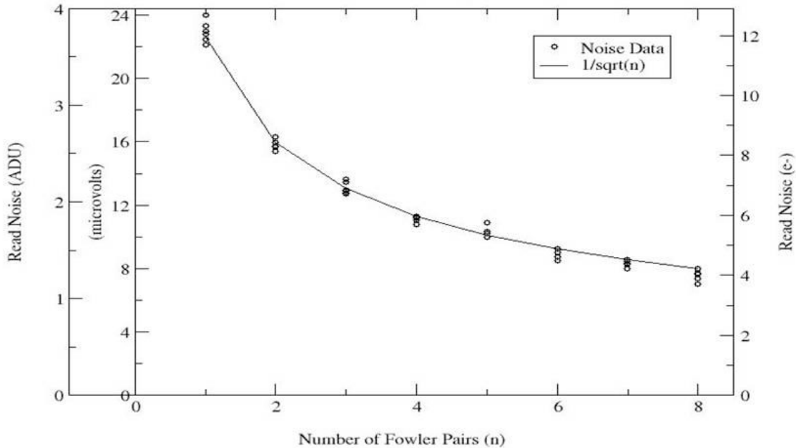
Fig. 9. Noise measured by University of Rochester on a Phoenix 2K × 2K InSb module using 100-second integrations. 1 The total noise—including readout, detector, and test set noise contributions—is shown as a function of the number of Fowler sample pairs. The noise follows the square root (number of Fowler pairs) relation predicted for uncorrelated white noise with 4 electrons noise measured for Fowler-8. The module temperature was 30 Kelvin.
