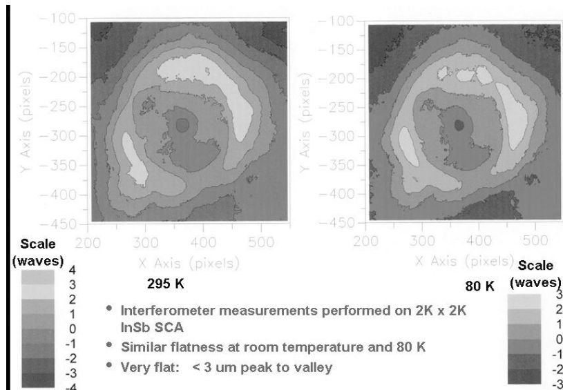
Fig. 6. Interferograms of the top surface of the detector on an ORION 2K \times 2K module. The picture on the left shows the flatness at 295 K while the flatness at 80 K is shown on the right. The scales (in waves) for the interferograms are included on each side. The detectors are extremely flat over this area and there is almost no change in shape with temperature.
