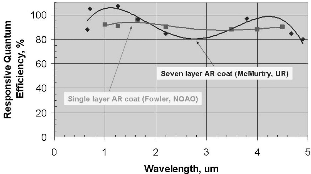
Fig. 7. QE of large-area InSb SCAs as a function of wavelength. The data obtained by Fowler at NOAO is from a 1\text{K} \times 1\text{K} ALADDIN SCA with a single-layer, broad-band AR coating. The data from McMurty at the University of Rochester is from a 2\text{K} \times 2\text{K} Phoenix SCA with a seven-layer AR coating designed to enhance visible response and maintain high QE in the infrared as well. The smooth curves are polynomial fits to each data set.
