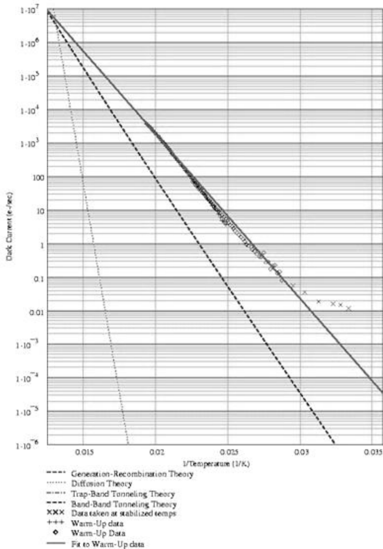
Fig. 11. Arrhenius plot of dark current as a function of inverse temperature for a 2K \times 2K InSb array obtained by the University of Rochester. 1 The measured dark current follows a straight line on this semi-log plot down to 33 K and then flattens out to 0.01 electrons/second at 30 K. Data were obtained both during warming up and cooling down the detectors.
