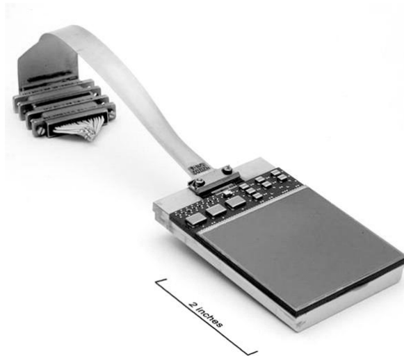
Fig. 8. The Phoenix 2048 × 2048 (2K × 2K) InSb module. The InSb SCA occupies the majority of the module surface. A temperature sensor, current-source resistors, and noise-reduction capacitors are located on the upper-left of the module.
