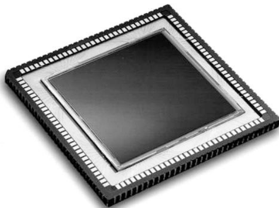
Fig. 3. ALADDIN InSb SCA with 1024 \times 1024 detector elements on 27 \mu\text{m} spacing. The SCA is mounted in a 124-pin leadless chip carrier (LCC).
