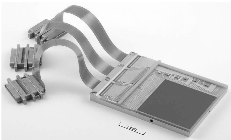
Fig. 4. An ORION 2048 \times 2048 ( 2\text{K} \times 2\text{K} ) InSb SCA mounted on a module. A temperature sensor and noise-reduction capacitors are also mounted on the module. Two of the connecting cables carry the 64 output lines; the third cable is for clocks and biases. Current sources for all 64 outputs, shown just to the left of the light-baffle bar, are included. The module is 2-side butttable.
