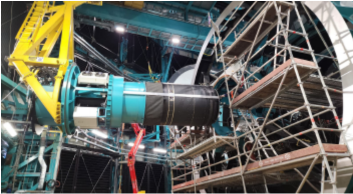
Figure 5: LSSTCam being lifted up for installation on the Simonyi Survey Telescope top end. The yellow lifting fixture is attached to the overhead dome crane and is being operated by lead mechanical engineer Freddy Muñoz in the boom lift (orange) behind the camera in this view (the person basket is not visible). The long aluminum bar (one of two) along the camera body is used to guide the camera through the secondary mirror (M2) hole visible at the center of the scaffolding. Credit: RubinObs/NOIRLab/SLAC/NSF/DOE/AURA
