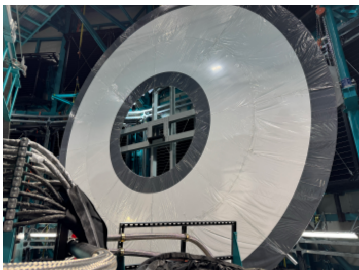
Figure 3: Rubin's large, reflective calibration screen mounted inside the dome. The screen is precision-made and aligned to provide a flat illumination of the focal plane used to calibrate LSSTCam images. Light sources project through the central hole toward the telescope, where a reflector sends the light back to fill the screen. This light then illuminates the telescope's mirrors and is directed into the camera. Credit: RubinObs/NOIRLab/SLAC/NSF/DOE/AURA
