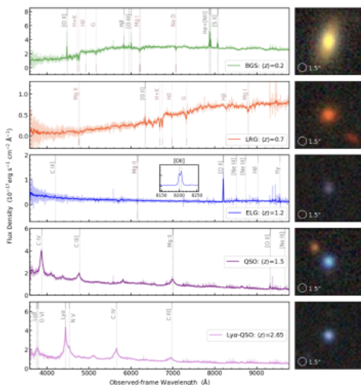
Figure 2: Composite spectra and example images of the DESI extragalactic target classes: Bright Galaxy Survey (BGS), Luminous Red Galaxy (LRG), Emission-Line Galaxy (ELG), and Quasi Stellar-Object (QSO). The latter are divided into tracer QSOs ( z < 2.1 ) and Lyman-alpha QSO ( z > 2.1 ). Each row shows the average of 75–100 spectra in a narrow redshift range around the labeled mean redshift value (left) and an image from the Legacy Surveys Sky Viewer for one representative example object (right). For the spectra, the faint colored lines represent the inverse-variance weighted average spectra, while the darker lines are the same spectra smoothed with a five-pixel Gaussian kernel. The vertical dotted lines indicate the expected wavelengths of key emission and absorption lines, and for the ELG class, the inset shows the resolved [O II] \lambda\lambda 3726, 29 Doublet. On the image panels, the 1.5 arcsecond diameter circles represent the size of the DESI fiber. Figure created using the Astro Data Lab and SPARCL, and reproduced from the DESI DR1 paper (DESI Collaboration et al. 2025).
