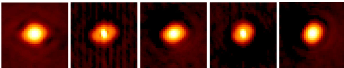
Figure 4: Speckle imaging time series of the asteroid Eros covering one rotation period (5.3 hours). During the series, the resolved shape of the non-spherical body is seen changing with time.
