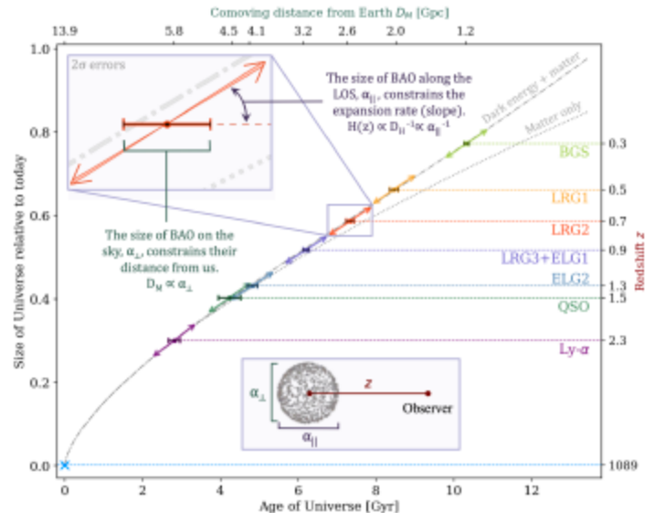
Figure 1: DESI’s BAO measurements constrain the expansion history of the Universe, shown here as the scale factor versus time. The angular size of the BAO signal measures the comoving distance to the sample (top horizontal axis). The size of BAO along the line-of-sight measures the Hubble distance, and therefore the expansion rate, or the slope on the curve. The scale factor is inferred from the effective redshift of the sample. DESI measures the BAO signal for seven tracer samples between redshifts of 0.5 to 2.3. The constraint from the CMB acoustic scale is plotted as a light blue cross. The late-time acceleration caused by dark energy is easily seen as favored by the BAO data. The bottom axis shows the age of the Universe as a function of comoving distance in a flat \Lambda CDM universe. DESI-fitted models with evolving dark energy are not visually distinguishable from the \Lambda CDM model on this plot. (Credit: Figure 1 from DESI Collaboration 2025)
