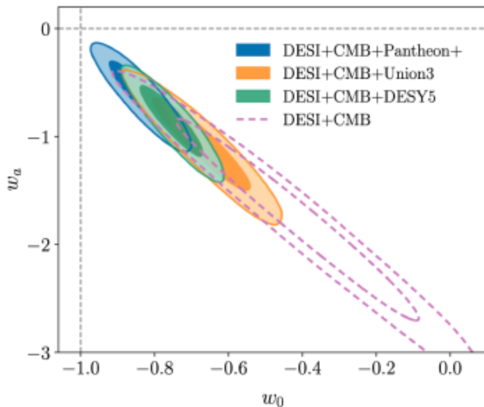
Figure 2: Best fit quantities describing the dark energy equation of state parameter w in a model that evolves as w(a) = w_0 + w_a(1-a) , where a = 1/(1+z) , from fits to DESI data in combination with constraints from the CMB and three supernova datasets. The contours enclose 68% and 95% of the posterior probability. The intersection of the gray dashed lines indicates the \Lambda CDM limit ( w_0 = -1 , w_a = 0 ). \Lambda CDM is rejected at 2.8\sigma , 3.8\sigma , and 4.2\sigma significance for DESI combined with the Pantheon+, Union3, and DES5 supernova samples, respectively, and 3.1\sigma for DESI+CMB without any supernovae. (Credit: Figure 11 from DESI Collaboration 2025 )
