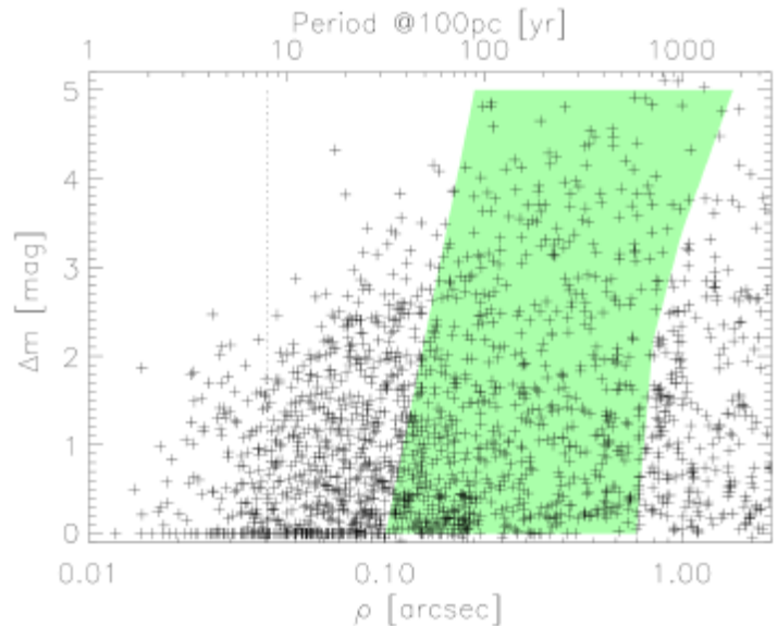
Figure 1: Magnitude difference m vs. separation for 1533 pairs measured at SOAR in 2023 (crosses). The upper axis indicates approximate periods of binaries with such separations located at 100 pc distance. The green shading highlights the expected future measurements from Gaia, the vertical dotted line shows the SOAR diffraction limit of 40mas in the I band (from Tokovinin et al. 2024).
