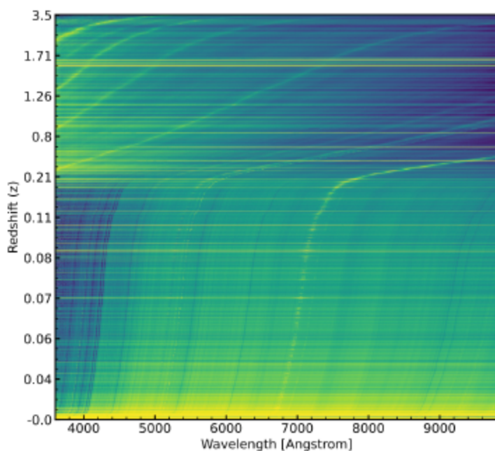
Figure 3: DESI spectra of 5687 primarily extragalactic sources from the Milky Way Backup Program, arranged in increasing redshift. Several emission and absorption features typical of galaxy and QSO spectra are seen tracking diagonally across the image with increasing redshift. Emission features appear lighter toward yellow colors while absorption features appear darker toward blue colors. A small number of the brightest horizontal lines are spectra of stars that are mis-classified as spectral type GALAXY by the default DESI pipeline. This figure was made by retrieving the spectra using CSDC's SPARCL and will be published as part of the DESI Backup Program Overview paper (Dey et al. 2025).
