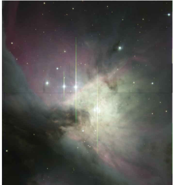
Figure 3: Image of the Orion Nebula, created by the 2025 REU/PIA students using the SMARTS-GSU 0.9-meter Telescope. (Credit: NOIRLab/NSF/AURA/2025 NOIRLab REU-PIA students/G. Damke)
