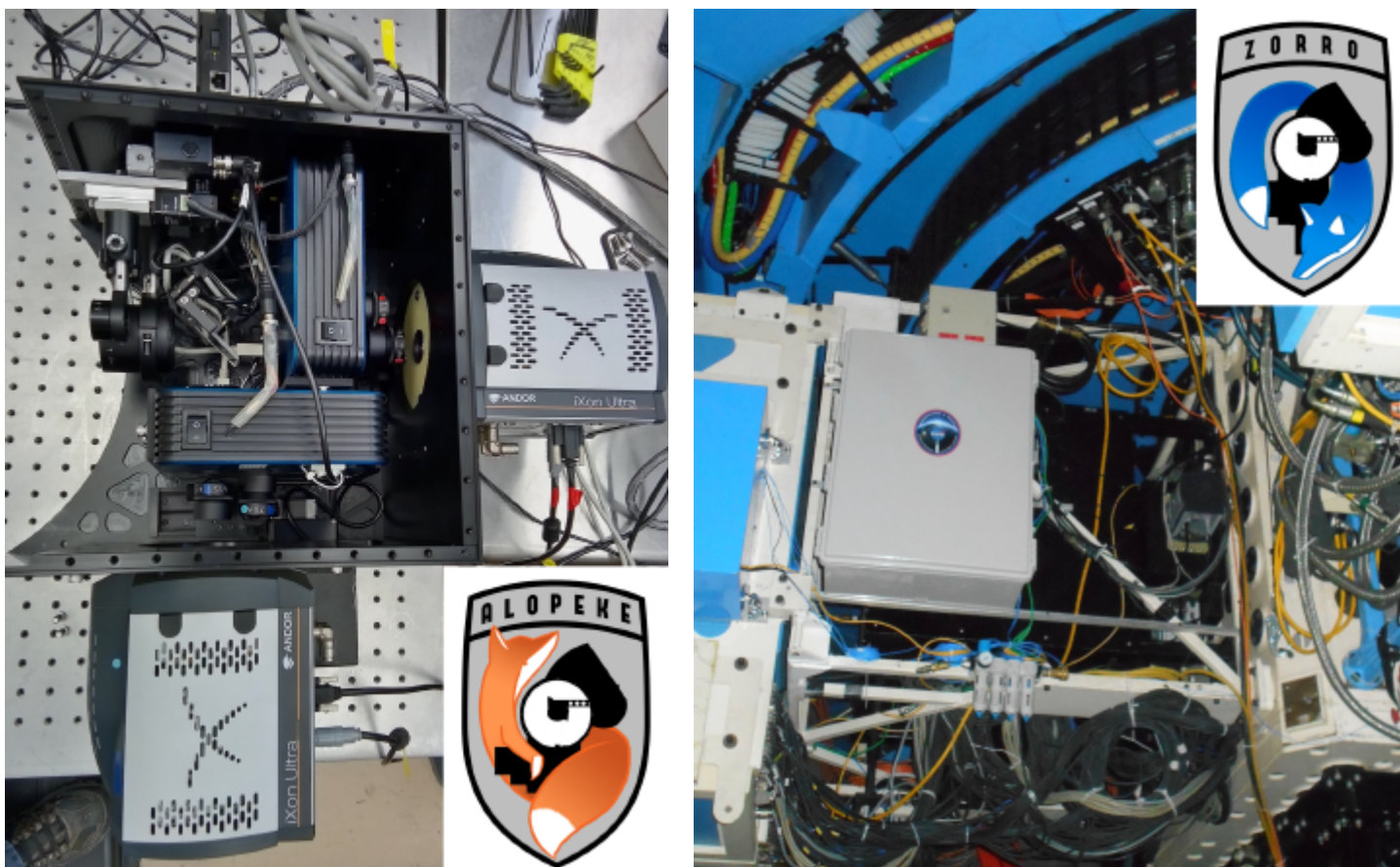
Figure 1: Left: The 'Alopeke instrument components were visible during a routine maintenance inspection at the Gemini North base facility. With the covers removed, one can see the tightly packed innards that contain two filter wheels, the optical elements, and the two ANDOR EMCCD cameras extending from the box. Right: Zorro mounted on the Gemini South telescope, in its permanent mount location at the GCAL port, attached underneath the primary mirror. The black box with one ANDOR EMCCD camera seen extending from it contains the instrument, while the larger white box to the left contains the electronic power supplies and instrument computer.
