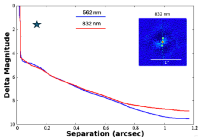
Figure 2: A typical speckle imaging result for an 8th magnitude star (TOI-5873). The red and blue curves show the 5\text{-}\sigma contrasts achieved as a function of angular separation, from the diffraction limit out to 1.2 arcsec, and the inset shows the reconstructed image for the 832-nm observation. The star symbol shows the location of the companion. The speckle observations reveal that the target star is binary, with a very close (0.14 arcsec separation) companion that is 1.6 mag fainter than the primary at a position angle of 176 degrees.
