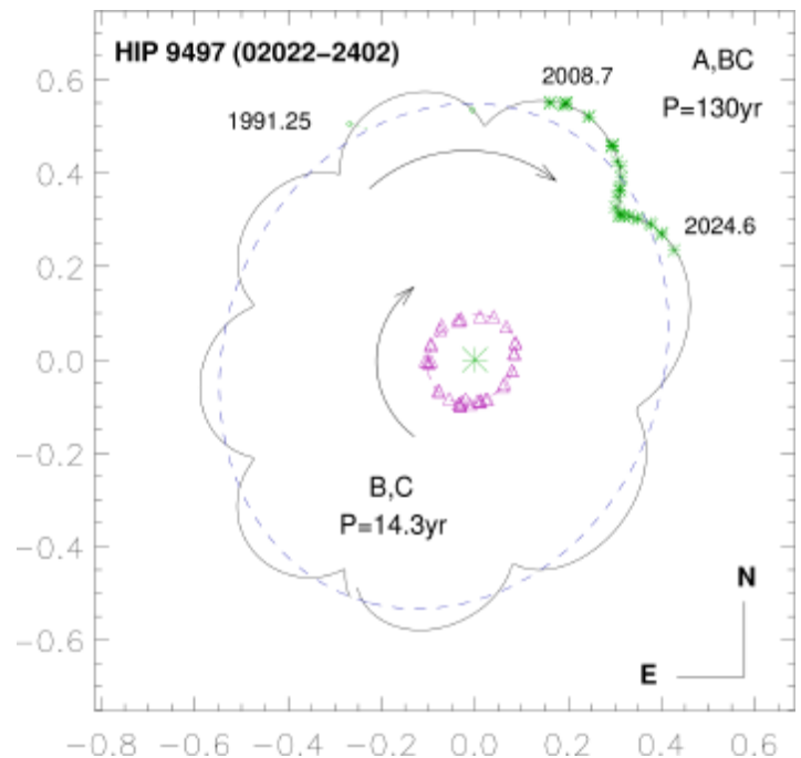
Figure 2: Orbital architecture of the hierarchical triple system HIP 9497 discovered at SOAR in 2008. The 14.3-yr orbit of the inner pair B,C is now fully covered (magenta symbols and ellipse), while the outer orbit (blue dash and black solid lines, green asterisks) with a period of 130 yr is known approximately. Both orbits are nearly circular and coplanar. The mass ratios in the inner and outer pairs are close to one. Such configuration is typical for many (but not all) low-mass triples.
