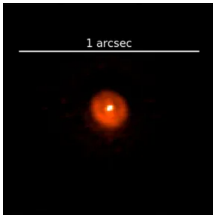
Figure 3: Nova V906 Car observed 978 days after its explosion. The image shows a resolved nova shell with a radius of 90 mas.
