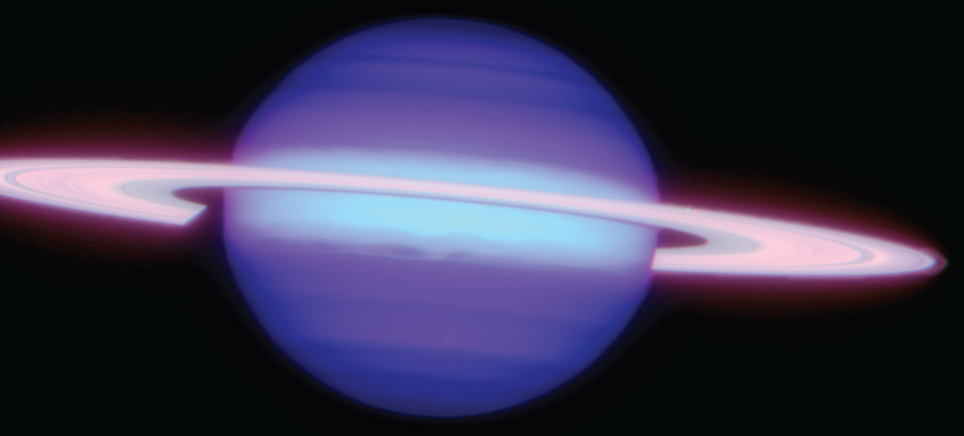
Saturn & Titan - NIRI / Altair AO - Gemini North
